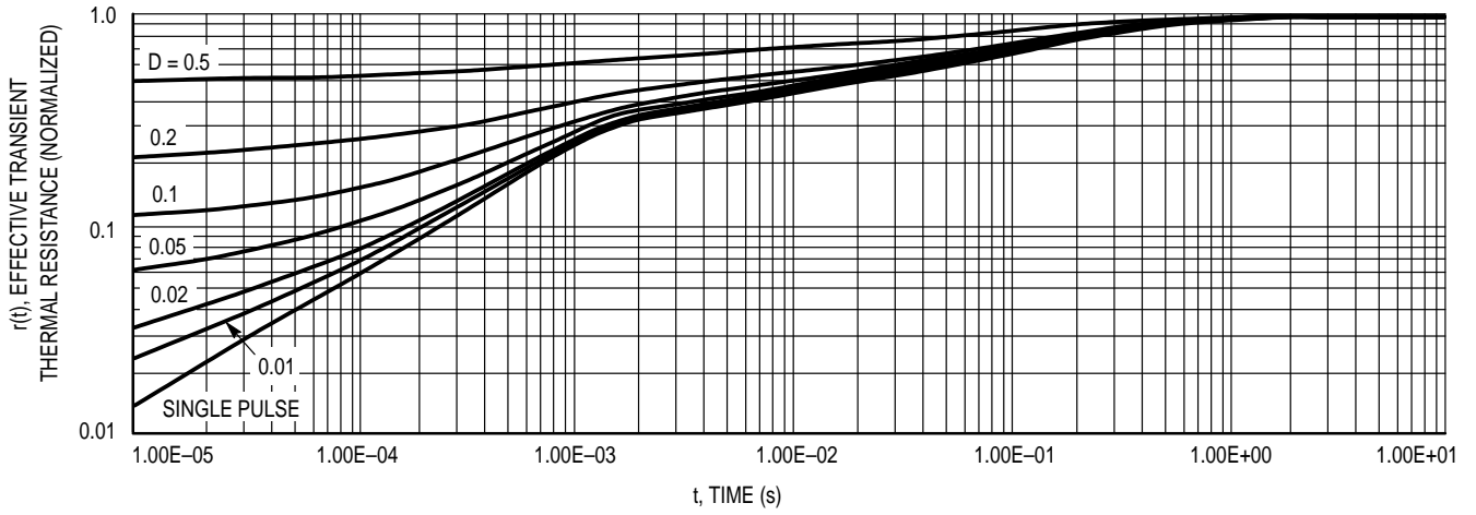
Figure 14. Thermal Response
